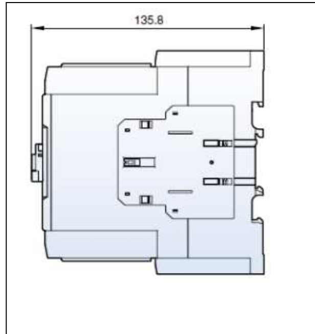
Contactor Dimension Comparison Dimensions in millimeters
