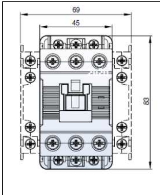
RSC-50 thru RSC-65
