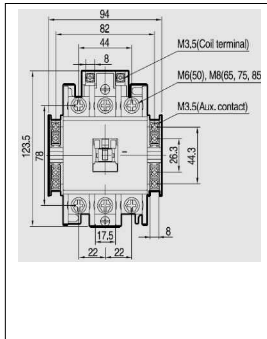
RSC-50 thru RSC-65
